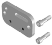
WC-AP Wheelchair attachment Adapter Plate MSRP: $28 Fits hole spacings between 1" to 2" (Plate size: 3" x 1.75" x .25")
