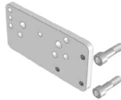
WC-AP2 Wheelchair attachment Adapter Plate 2 MSRP: $28 Fits Permobil Corpus and Koala hole spacing; use w/ Quantum or Jazzy w/c tie downs (Plate size: 3.5" x 2.25" x .25)
