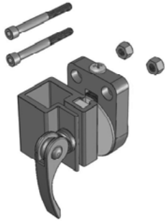
WB Wheelchair Bracket MSRP: $111 Angle and height adjustment for the post
